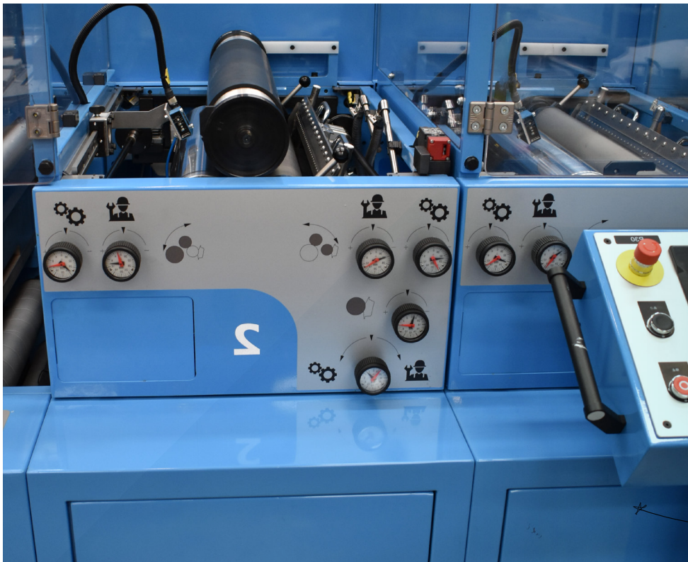
Printing Station
